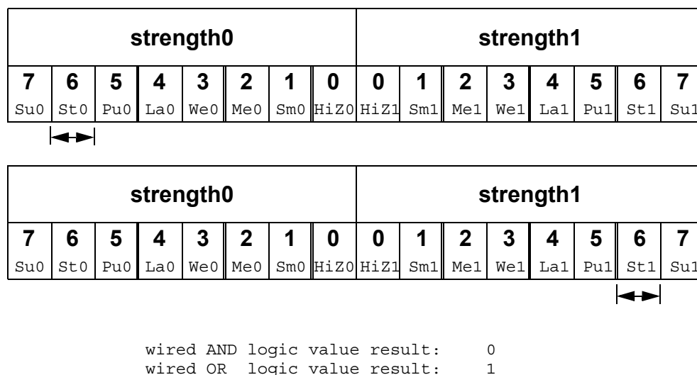
Figure 7-24—Wired logic with unambiguous strength signals
